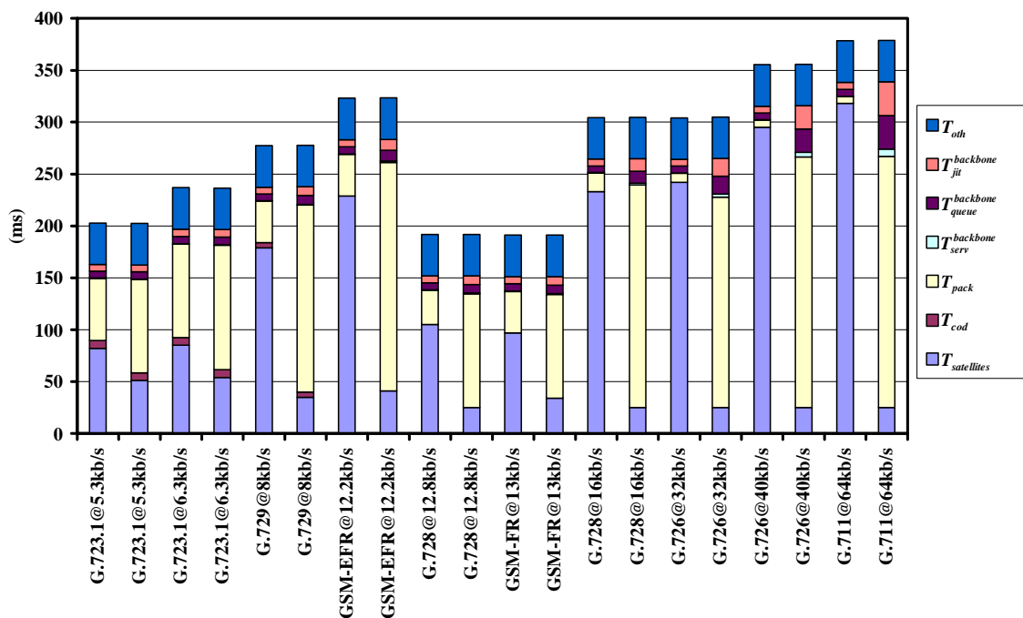
Figure 2: Decomposition of the tolerable M2E delay budget for the cases considered in Table 2.
