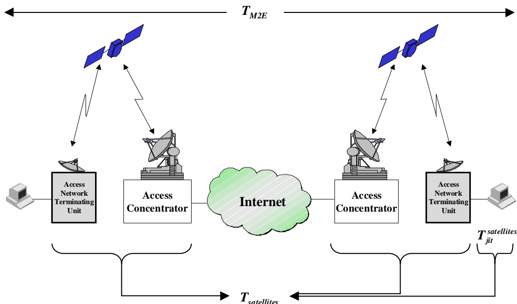
Figure 1: The satellite PC-to-satellite PC VoIP scenario.
